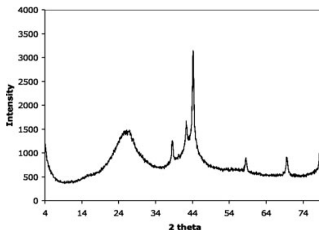
Figure 11. X-ray diffraction pattern of Ru/B- and N-doped microporous carbon.
