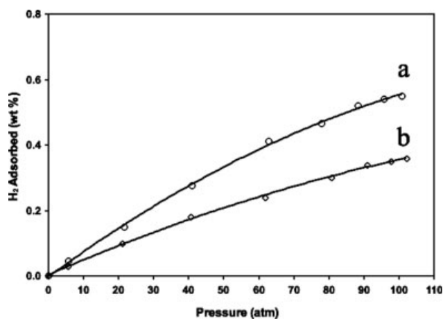
Figure 9. High-pressure hydrogen isotherms at 298 K for B- and N-doped microporous carbon (a: ○) and porous carbon CMK-3 (b: ◇).
