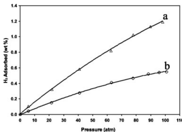
Figure 15. High-pressure hydrogen isotherms at 298 K on Ru/B- and N-doped microporous carbon (a: \Delta ) and B- and N-doped microporous carbon (b: \circ ).
